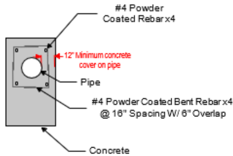
CONCRETE ENCASEMENT DETAIL
